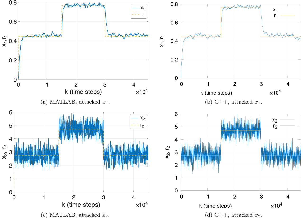
Figure 17: Attacked CSTR state trajectories (std = 2): MATLAB (left) vs. C++ (right). Both exhibit the same tracking degradation pattern.
